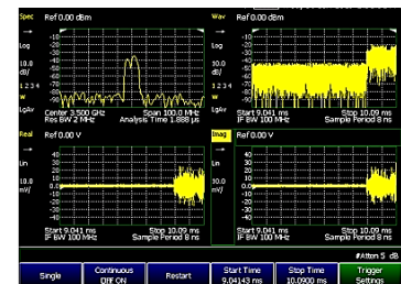
IQ data captured in FieldFox I/Q analyzer mode
