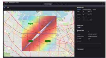
TDoA by three FieldFox
